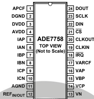
Figure 5. Pin Configuration
